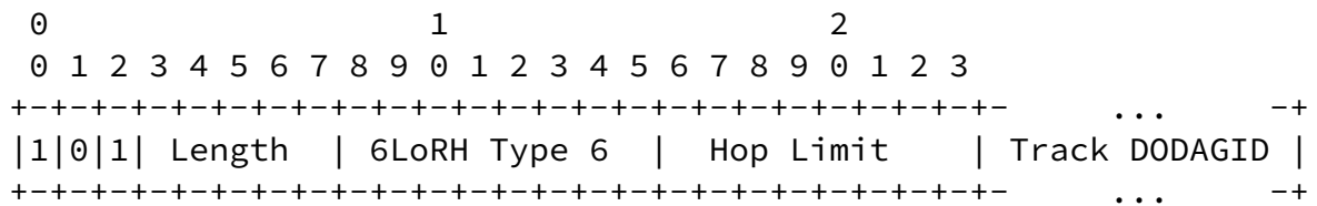
Figure 21: The IP-in-IP 6LoRH Header
