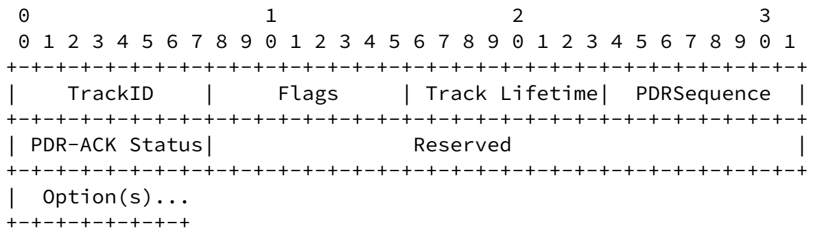
Figure 14: New PDR-ACK Control Message Format
