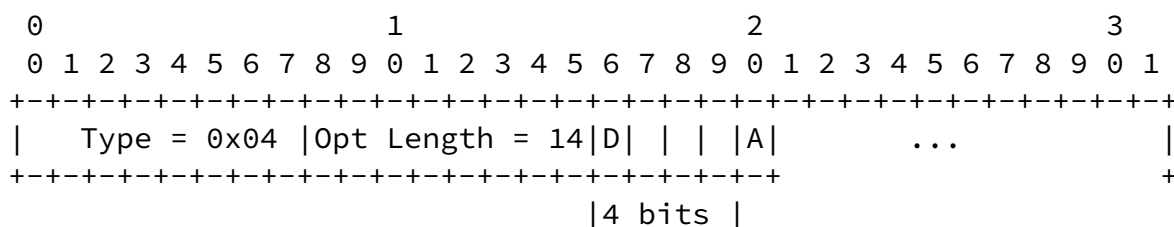
Figure 10: DODAG Configuration Option (Partial View)
