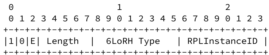
Figure 12: P-RPI-6LoRH Format
