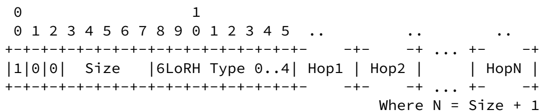
Figure 22: The SRH 6LoRH Header
