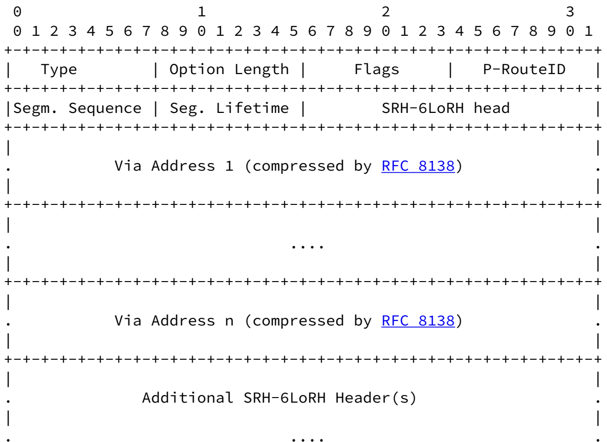
Figure 16: VIO format (uncompressed form)
