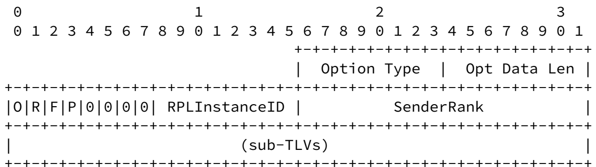
Figure 11: Extended RPL Option Format
