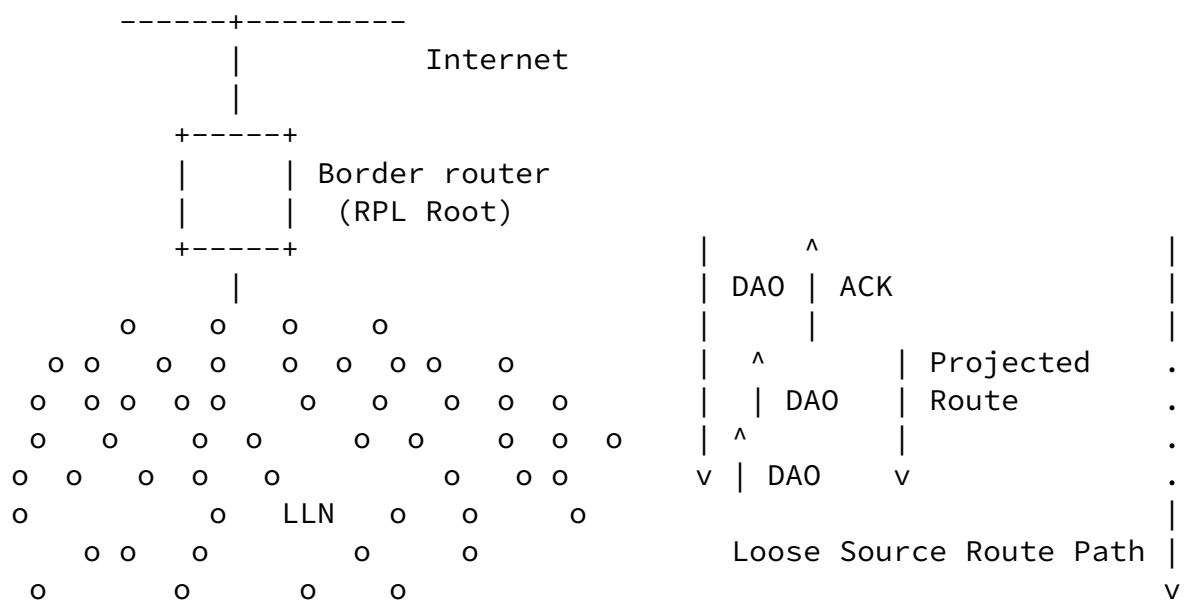
Figure 18: Projecting a route
