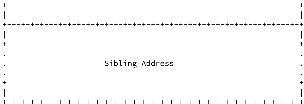
Figure 17: Sibling Information Option Format
