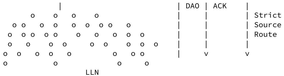
Figure 2: RPL Non-Storing Mode of operation
