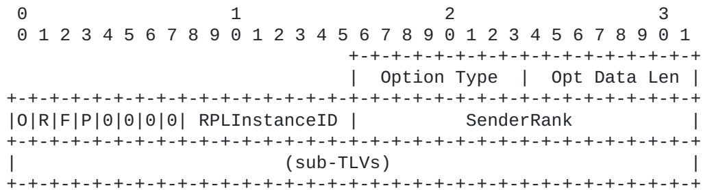
Figure 11: Amended RPL Option Format
