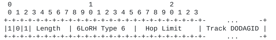
Figure 21: The IP-in-IP 6LoRH Header
