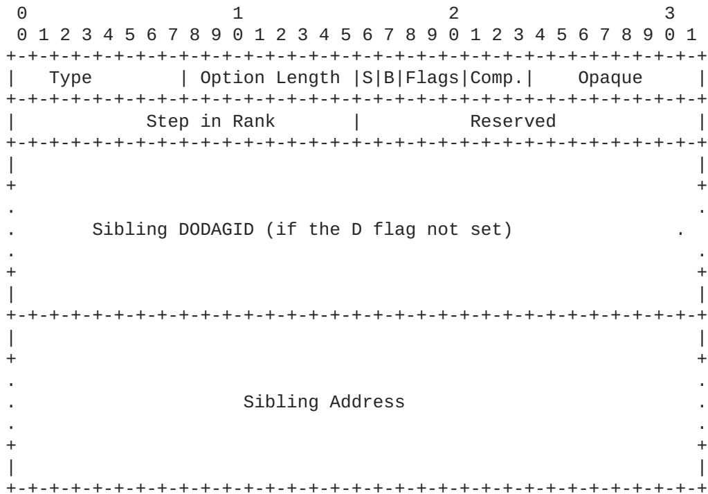
Figure 17: Sibling Information Option Format
