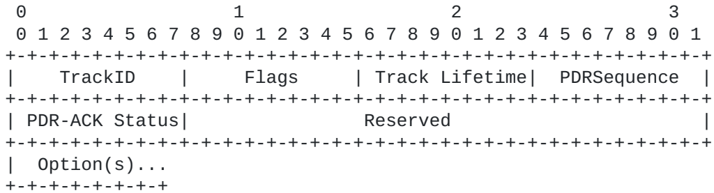
Figure 14: New PDR-ACK Control Message Format
