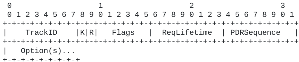
Figure 13: New P-DAO Request Format
