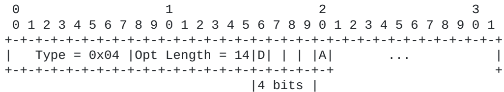
Figure 10: DODAG Configuration Option (Partial View)
