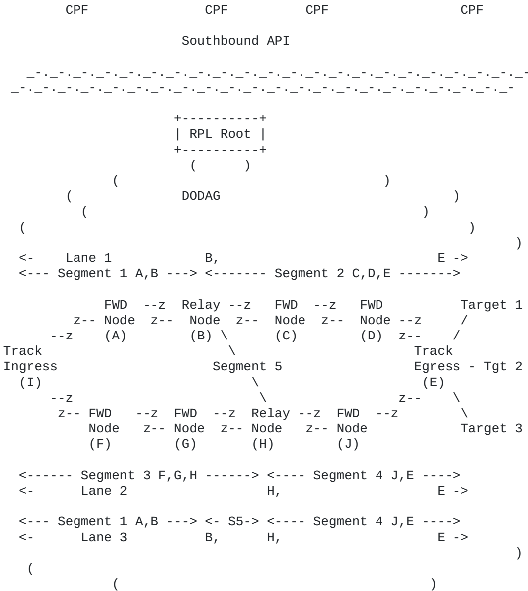
Figure 7: Segments and Tracks
