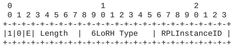
Figure 12: P-RPI-6LoRH Format
