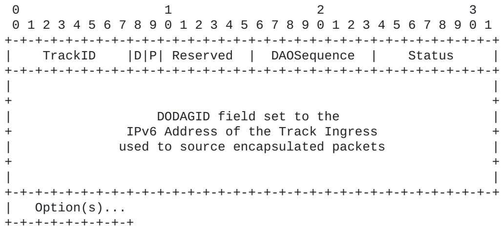
Figure 9: Projected DAO-ACK Base Object
