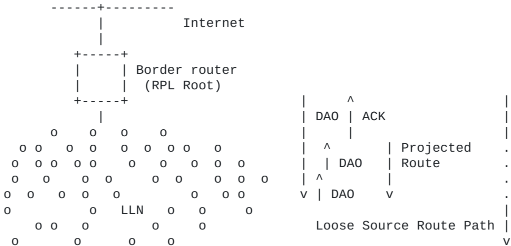
Figure 18: Projecting a route
