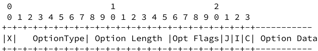
Figure 2: Extended RPL Option Format
