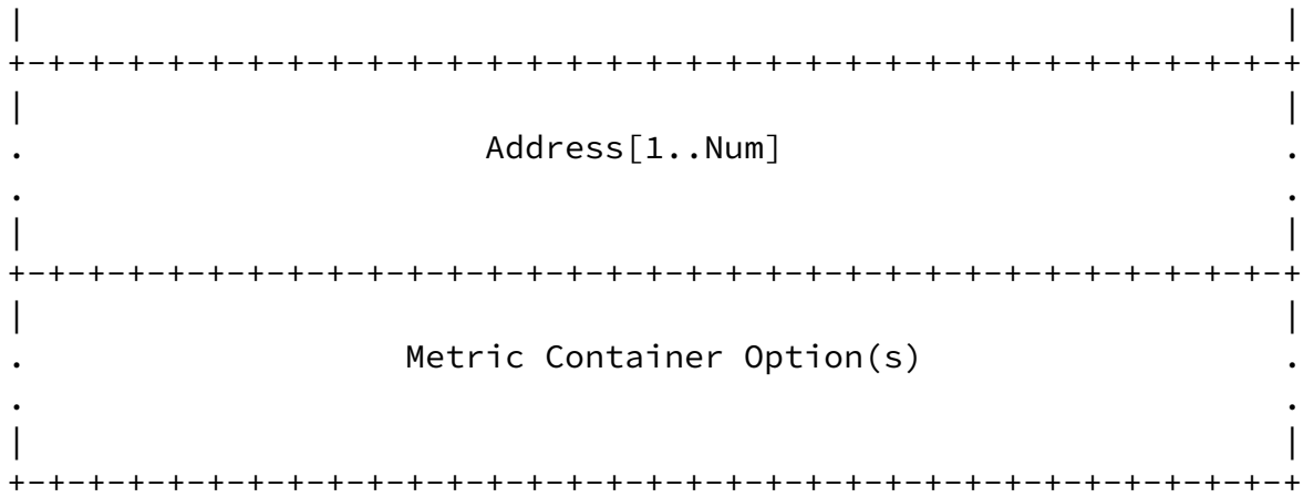
Figure 1: Format of the base Measurement Object (MO)
