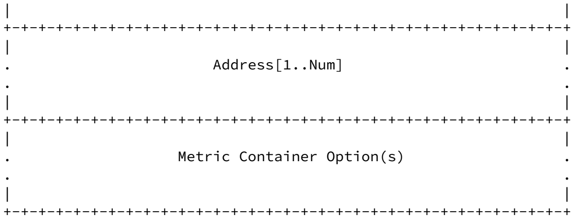
Figure 1: Format of the base Measurement Object (MO)
