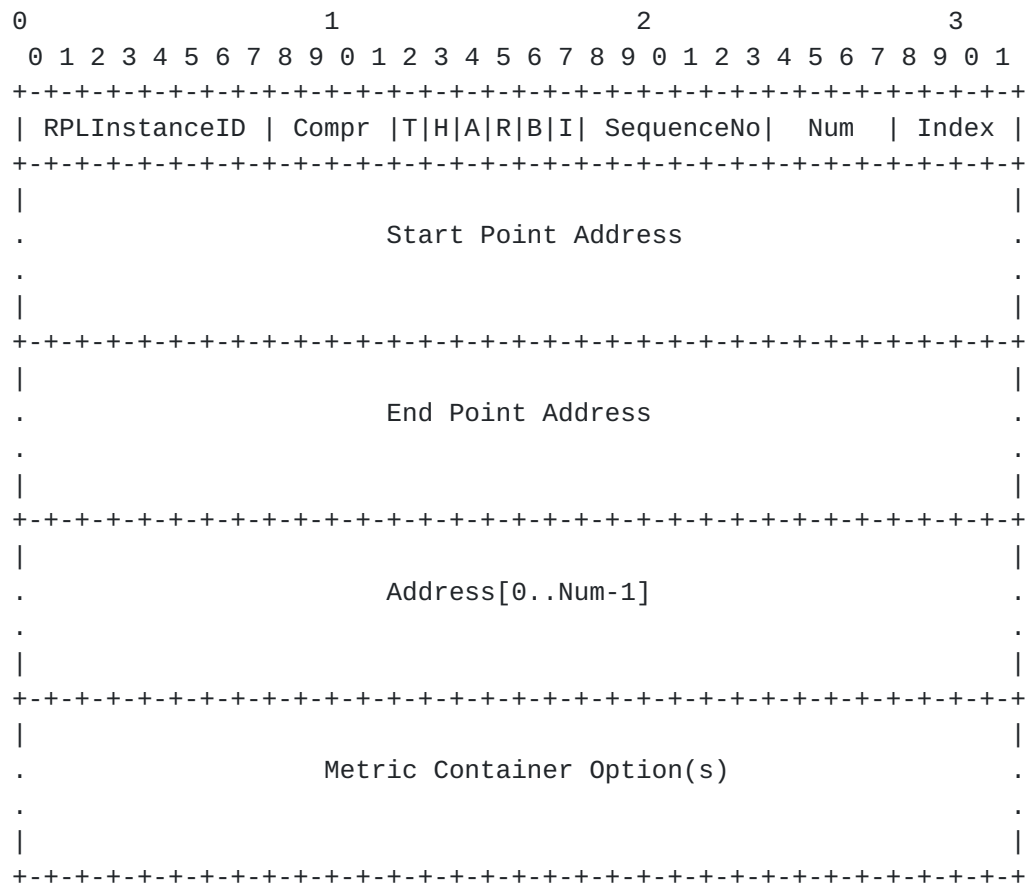
Figure 1: Format of the base Measurement Object (MO)
