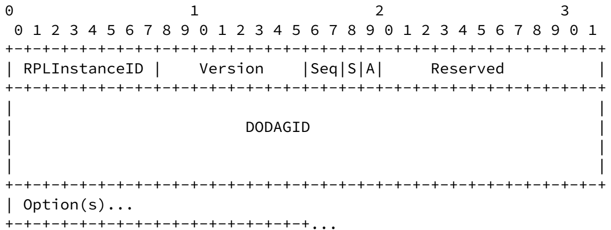
Figure 2: Format of the base Discovery Reply Object (DRO)
