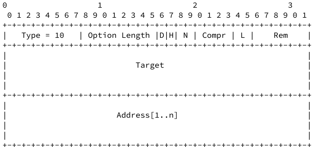
Figure 1: Format of the Route Discovery Option
