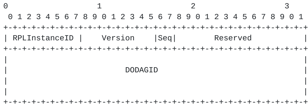
Figure 4: Format of the base Discovery Reply Object Acknowledgement (DRO-ACK)
