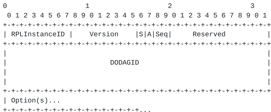
Figure 3: Format of the base Discovery Reply Object (DRO)
