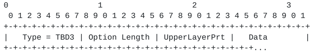
Figure 2: Format of Data Option
