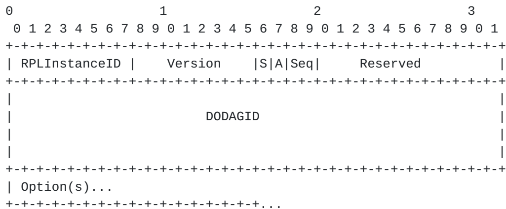
Figure 3: Format of the base Discovery Reply Object (DR0)
