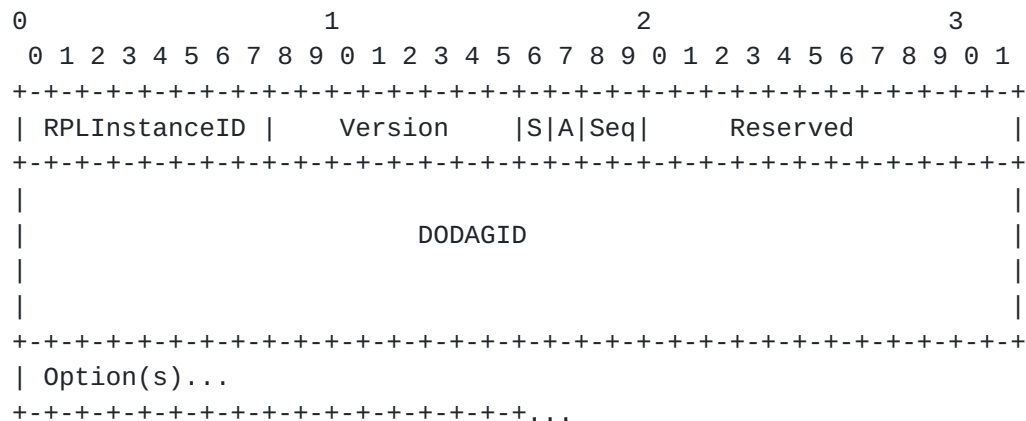
Figure 2: Format of the base P2P Discovery Reply Object (P2P-DR0)
