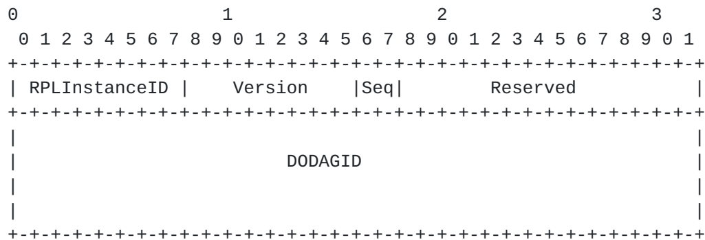
Figure 3: Format of the base P2P Discovery Reply Object Acknowledgement (P2P-DR0-ACK)
