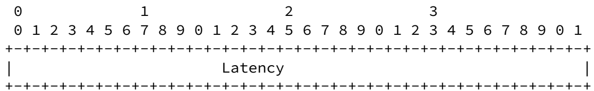
Figure 10: Latency Sub-object format
