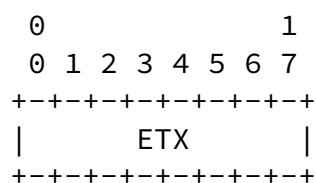
Figure 15: ETX Sub-object format
