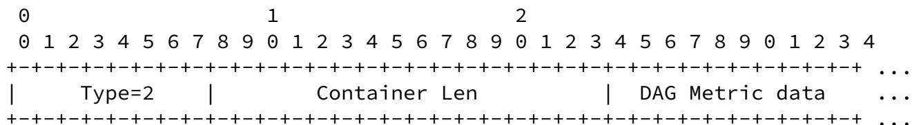
Figure 1: DAG Metric Container Format
