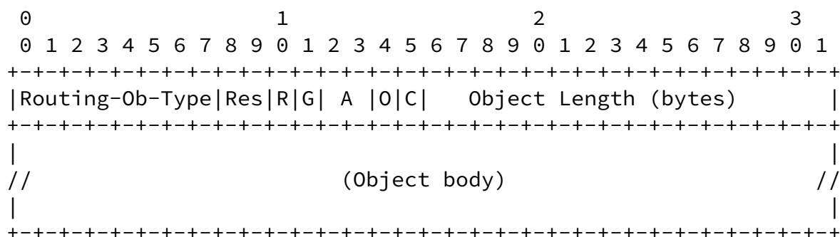
Figure 2: Routing Metric/Constraint common header format
