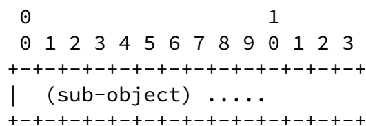
Figure 14: ETX Object Body Format
