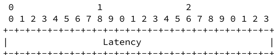
Figure 10: Latency Sub-object format
