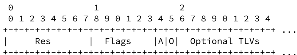
Figure 3: NSA Object format
