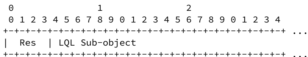
Figure 11: LQL Object format
