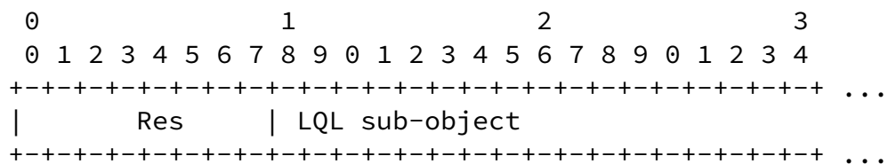
Figure 12: LQL object format
