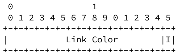
Figure 19: LC Type 2 sub-object format
