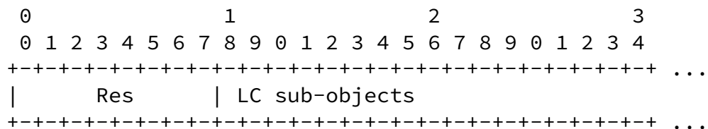
Figure 17: LC object format
