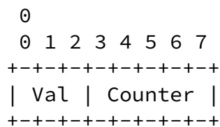
Figure 13: LQL Type 1 sub-object format
