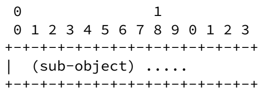
Figure 15: ETX object body format
