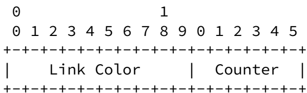
Figure 18: LC Type 1 sub-object format
