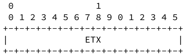
Figure 16: ETX sub-object format
