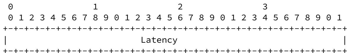
Figure 11: Latency sub-object format
