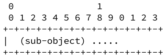
Figure 15: ETX object body format
