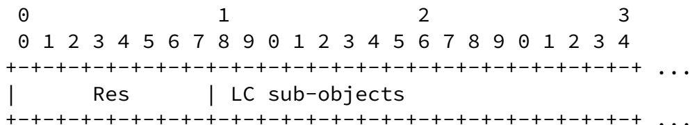
Figure 17: LC object format
