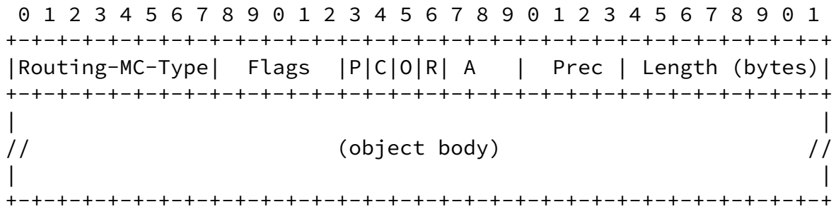
Figure 2: Routing Metric/Constraint object generic format
