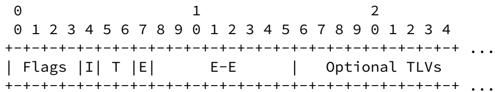
Figure 5: NE sub-object format
