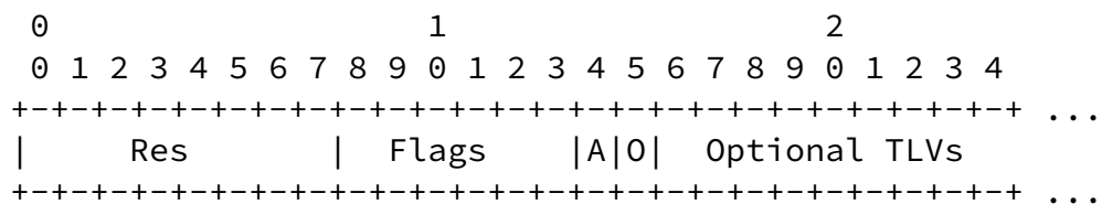
Figure 3: NSA object body format
