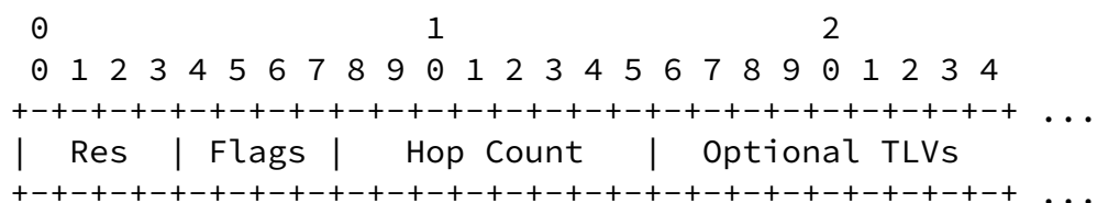
Figure 6: Hop Count object body format
