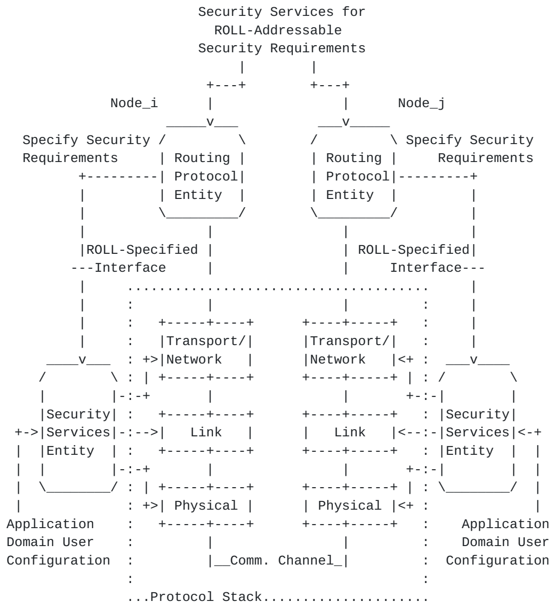
Figure 3: LLN Device Security Model
