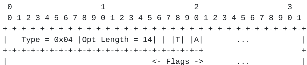
Figure 1: DODAG Configuration Option (Partial View)
