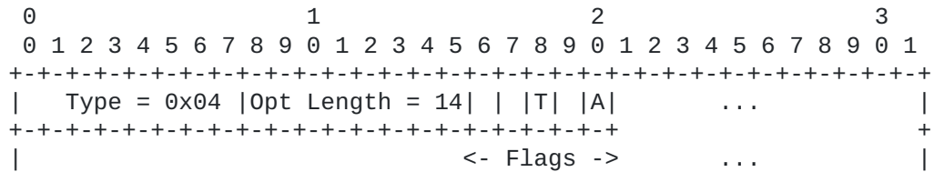
Figure 1: DODAG Configuration Option (Partial View)
