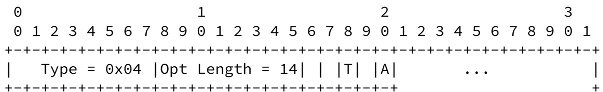
Figure 1: DODAG Configuration Option (Partial View)
