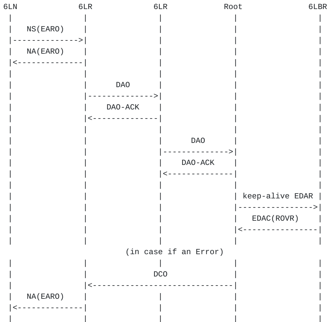
Figure 6: Next Registration Flow in Storing Mode
