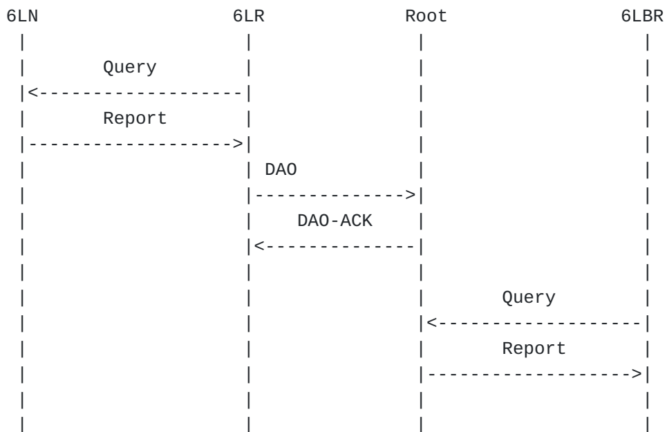
Figure 8: Next Registration Flow
