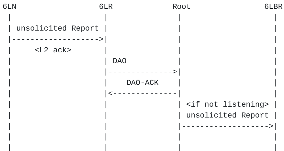
Figure 7: First Multicast Registration Flow
