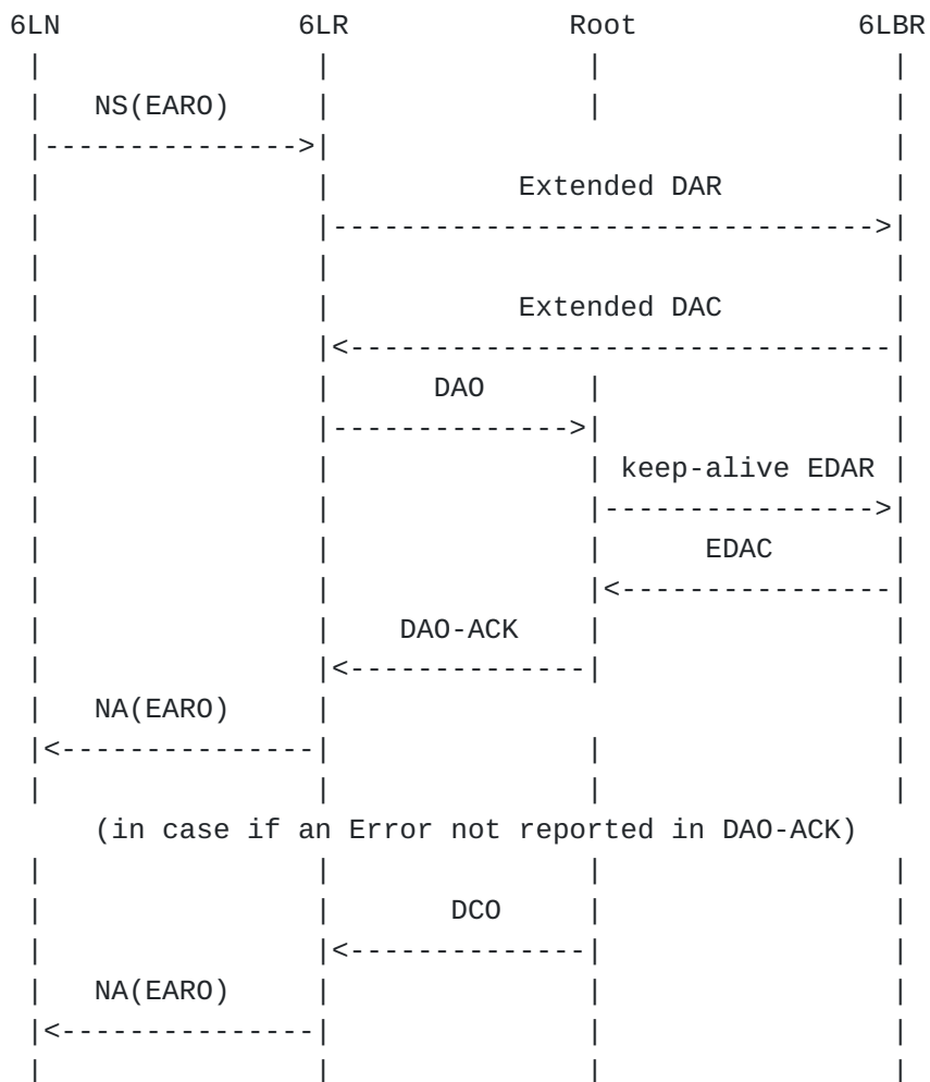
Figure 4: First Registration Flow in Non-Storing Mode
