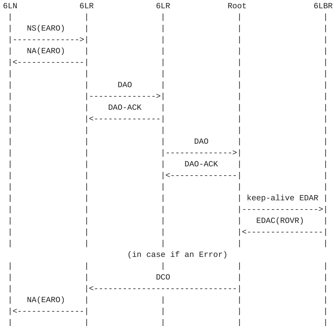
Figure 6: Next Registration Flow in Storing Mode
