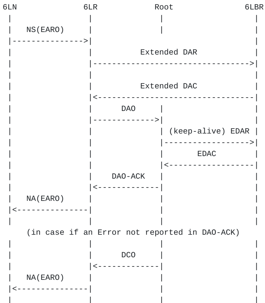
Figure 4: First Registration Flow in Non-Storing Mode
