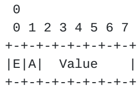
Figure 2: RPL Status Format
