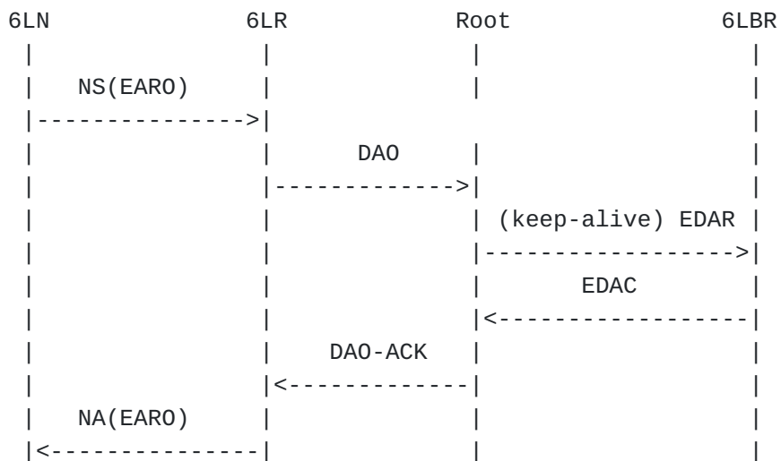
Figure 5: Next Registration Flow in Non-Storing Mode
