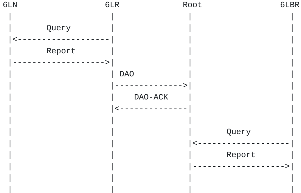
Figure 9: Next Registration Flow
