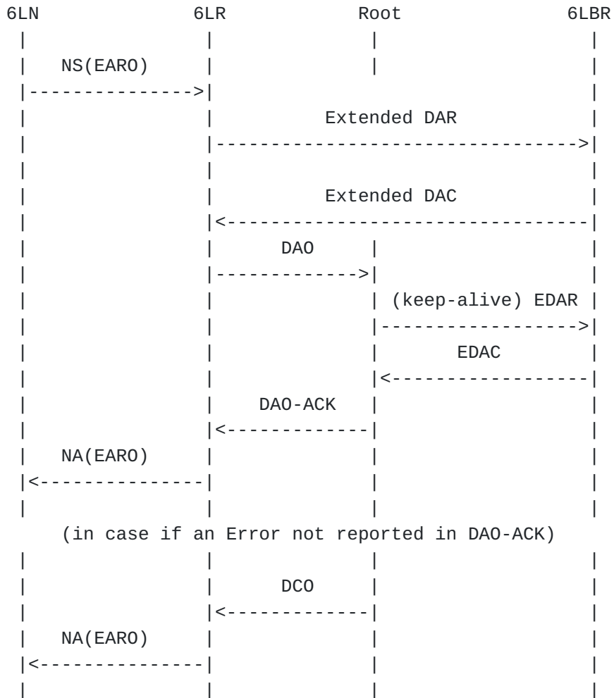
Figure 5: First Registration Flow in Non-Storing Mode
