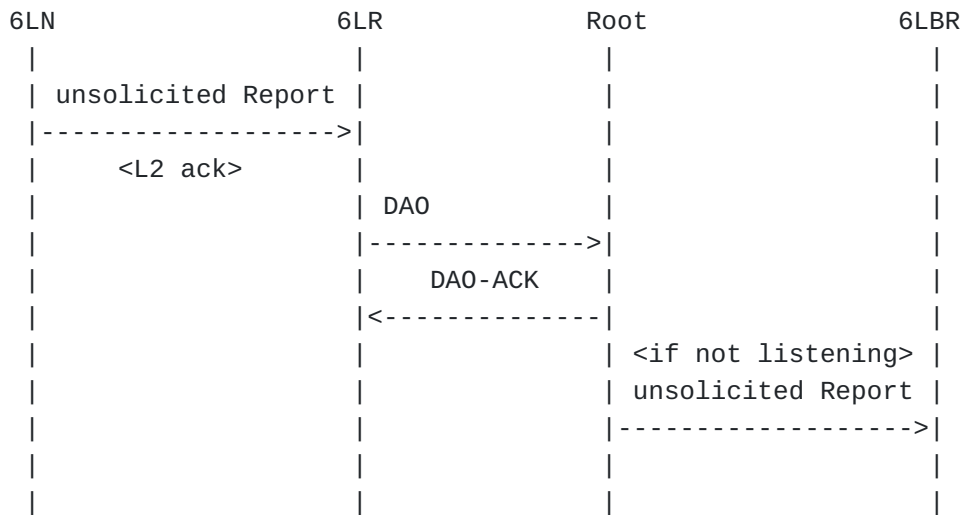
Figure 8: First Multicast Registration Flow
