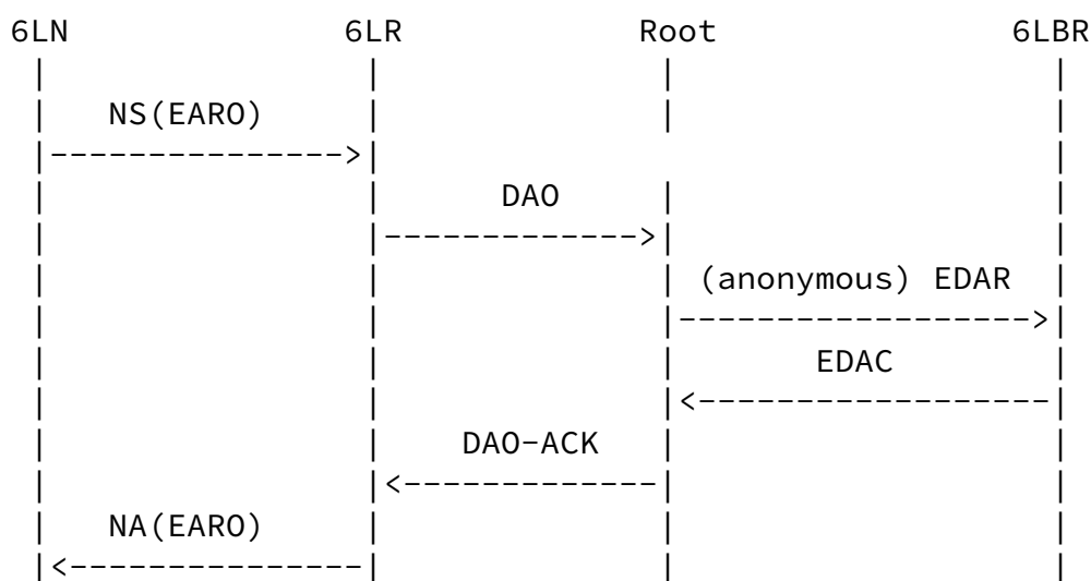
Figure 7: Next Registration Flow in Non-Storing Mode
