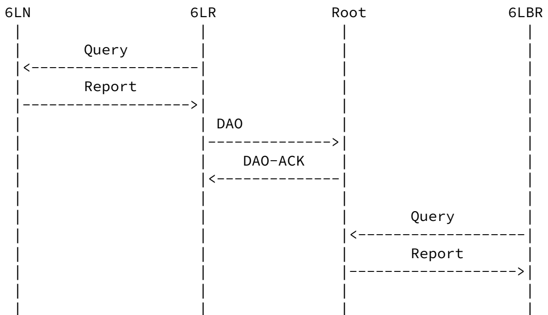
Figure 11: Next Registration Flow
