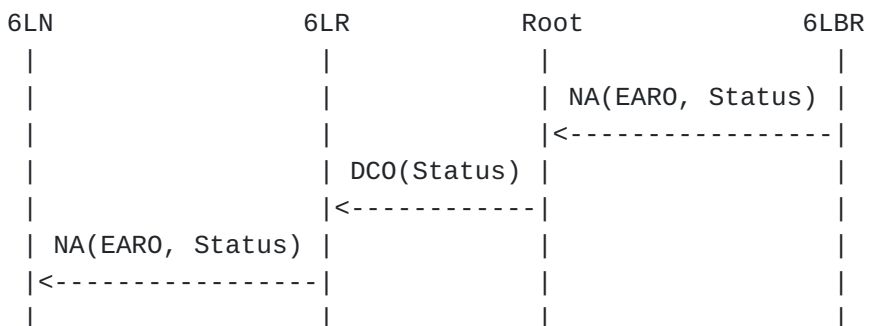
Figure 6: Asynchronous Issue
