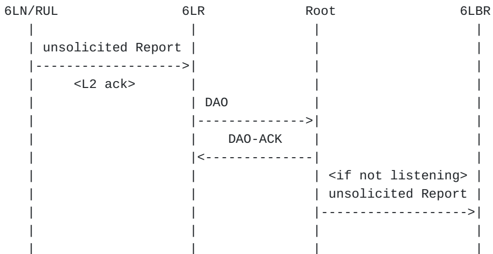
Figure 10: First Multicast Registration Flow
