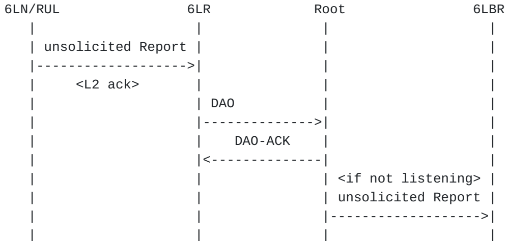
Figure 8: First Multicast Registration Flow
