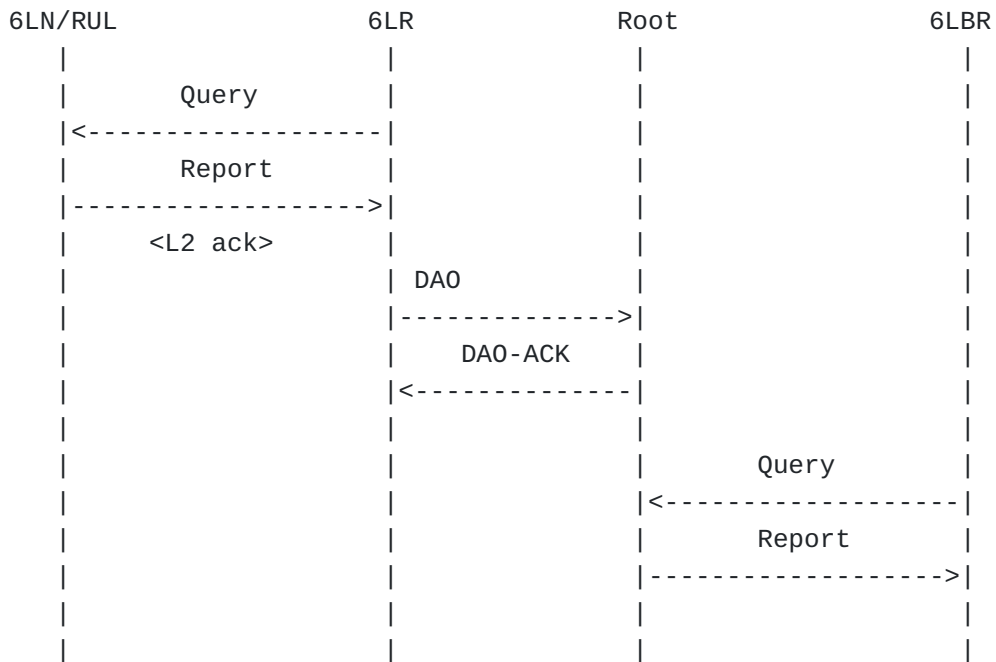
Figure 9: Next Registration Flow
