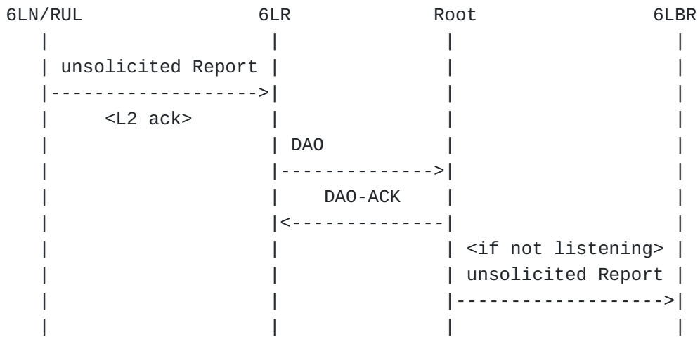
Figure 8: First Multicast Registration Flow
