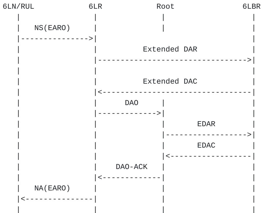
Figure 5: First RUL Registration Flow
