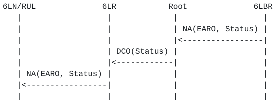
Figure 6: Asynchronous Issue
