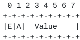
Figure 3: RPL Status Format
