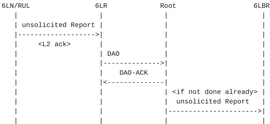
Figure 10: First Multicast Registration Flow
