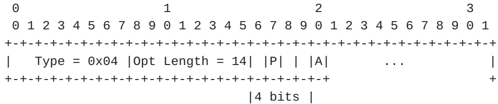
Figure 5: DODAG Configuration Option (Partial View)
