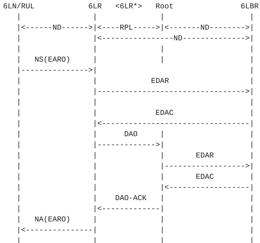
Figure 7: First RUL Registration Flow
