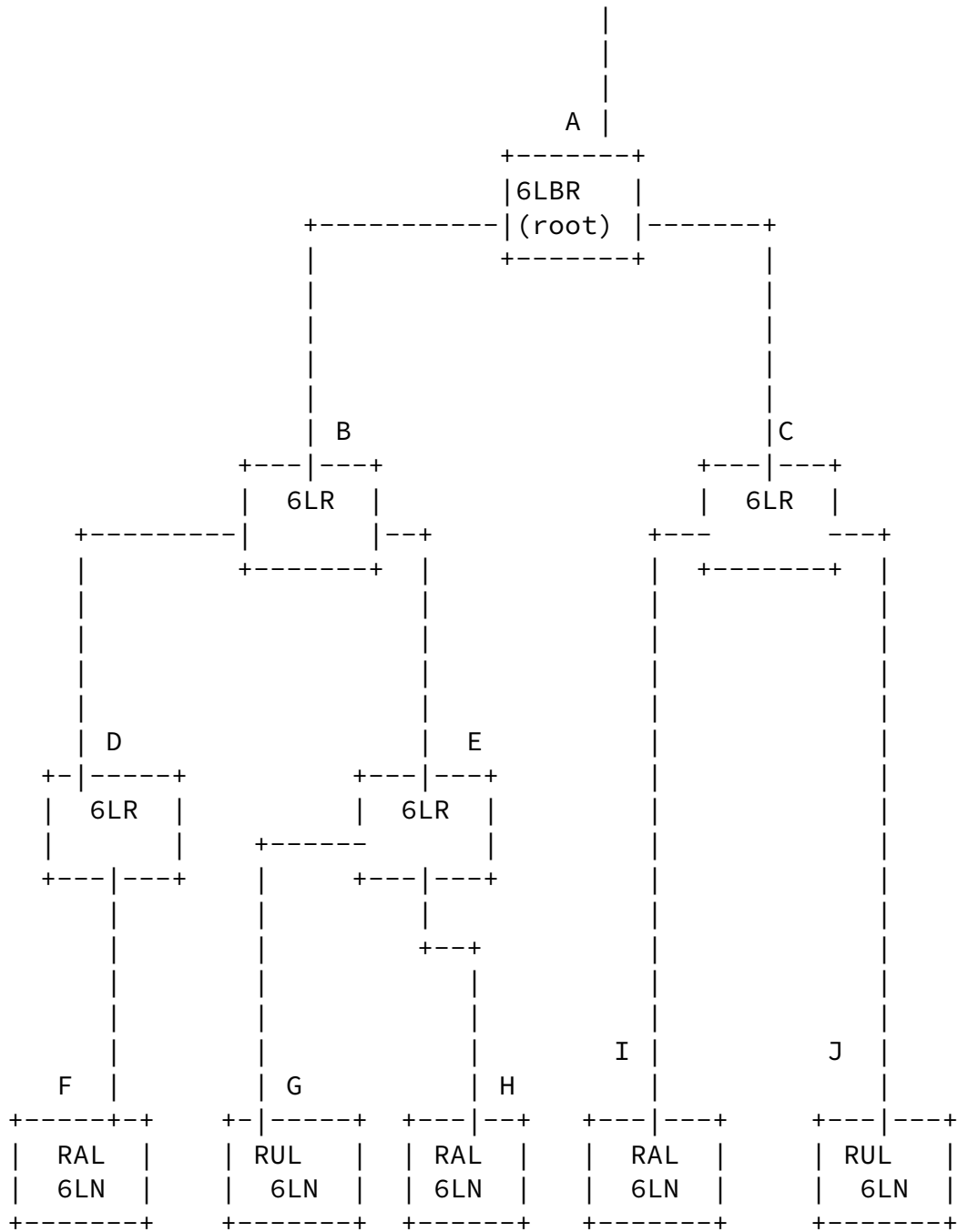
Figure 6: A reference RPL Topology.
