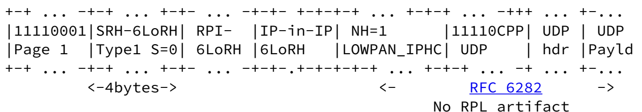
Figure 5: RPI Inserted by the Root in Storing Mode
