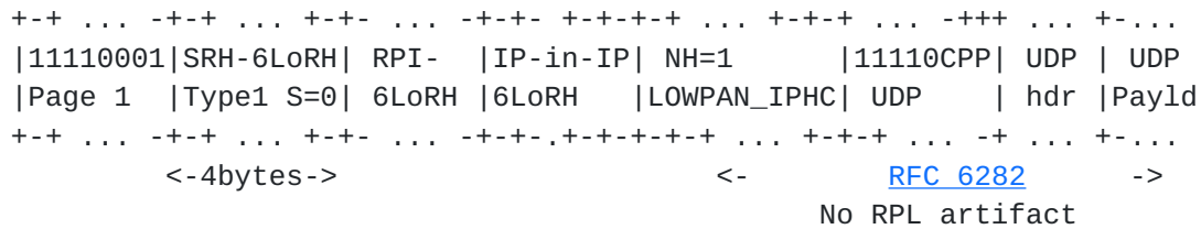
Figure 5: RPI Inserted by the Root in Storing Mode
