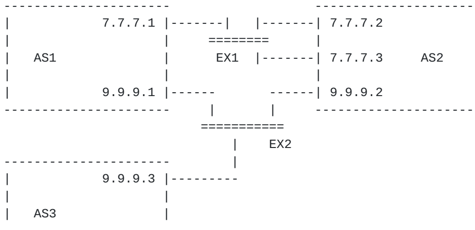
Figure 22: Example topology consisting of three ASes, AS1, AS2, and AS3; two exchange points, EX1 and EX2; and six routers.
