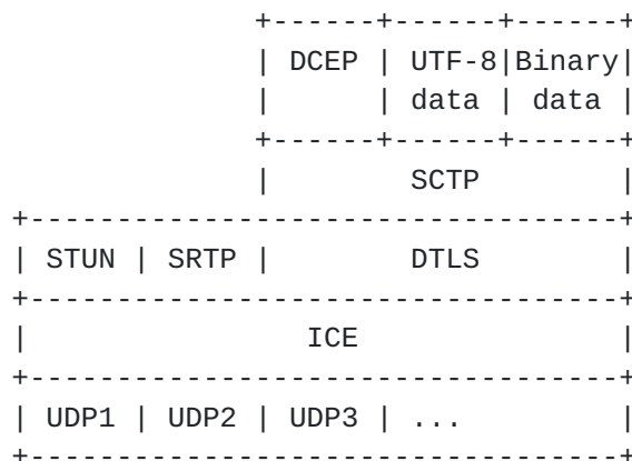
Figure 2: WebRTC protocol layers
