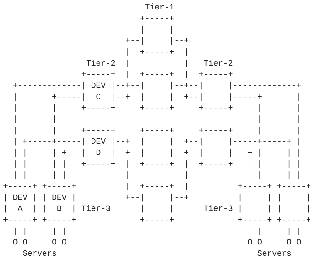
Figure 3: 5-Stage Clos topology
