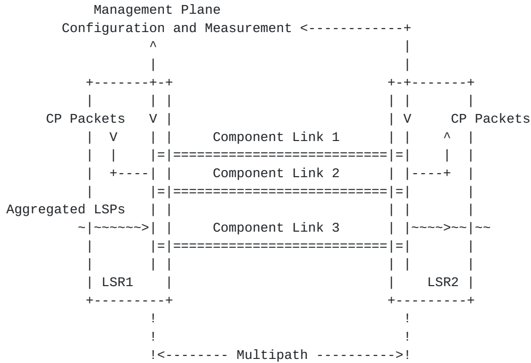
Figure 1: a multipath constructed with multiple physical links between two LSR
