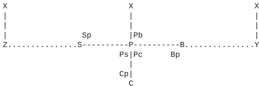
Figure 3: Multi-homed Prefixes
