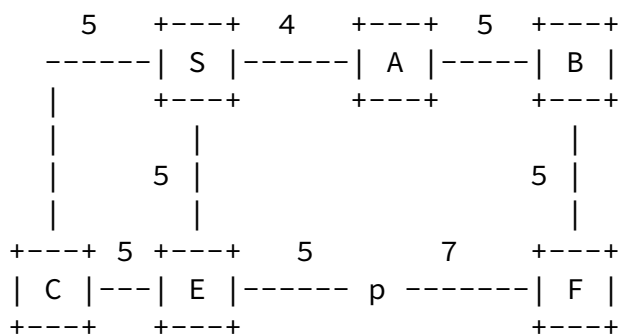
Figure 6: Multi-homed prefix
