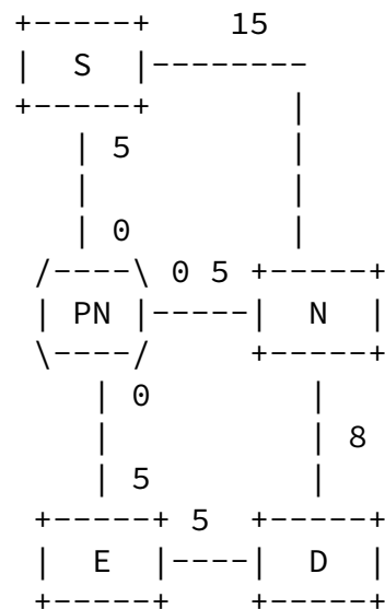
Figure 3: Loop-Free Alternate that is Link-Protecting
