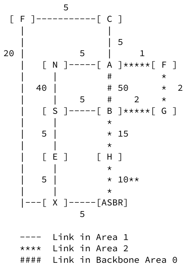
Figure 7: Topology with Multi-area ASBR Causing Area Transiting
