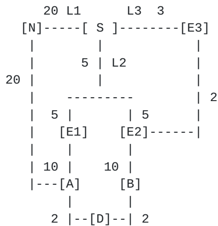
Figure 4: ECMP where Primary Next-Hops Provide Limited Protection
