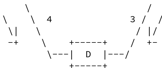
Figure 1: Basic Topology
