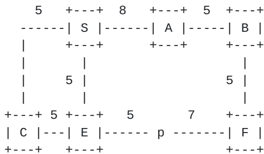
Figure 6: Multi-homed prefix
