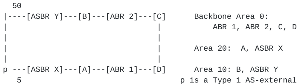
Figure 4: AS external prefixes in different areas
