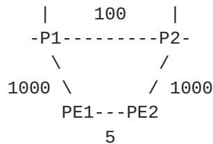
Figure 3: Example SP topology
