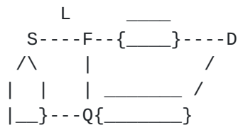
Figure 2: TI-LFA Protection
