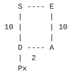
Figure 1 - Network topology suffering from micro-loops
