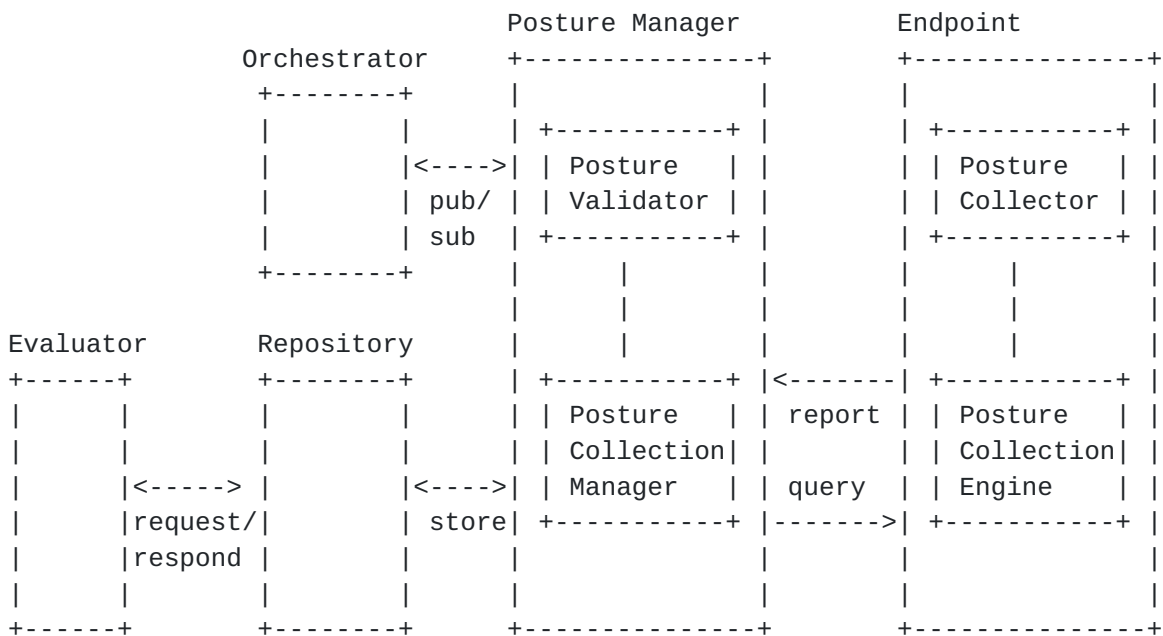
Figure 1: ECP Components
