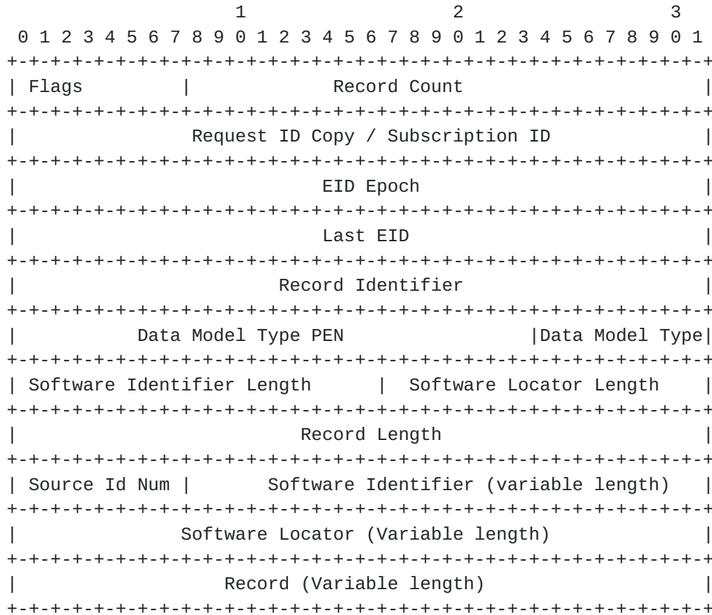
Figure 9: Software Inventory Attribute
