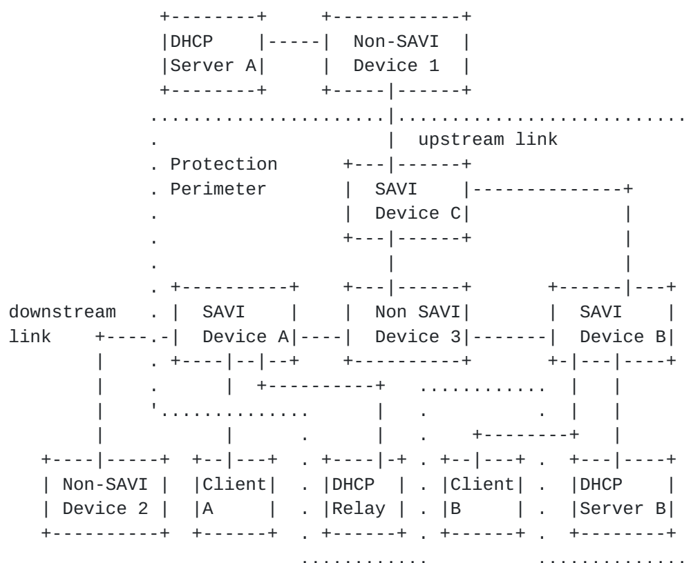
Figure 1: SAVI-DHCP Scenario
