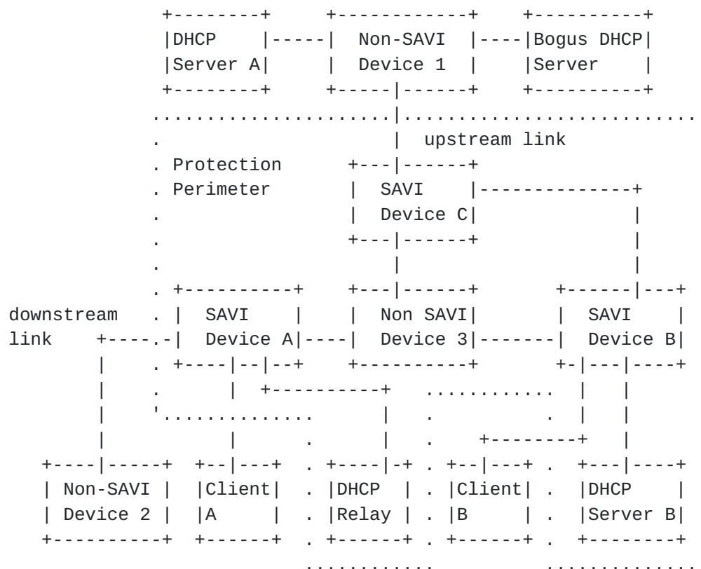
Figure 1: SAVI-DHCP Scenario
