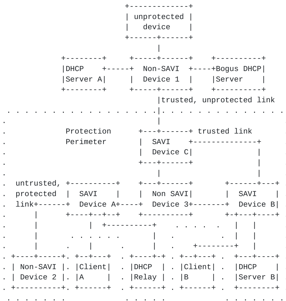
Figure 1: SAVI-DHCP Scenario
