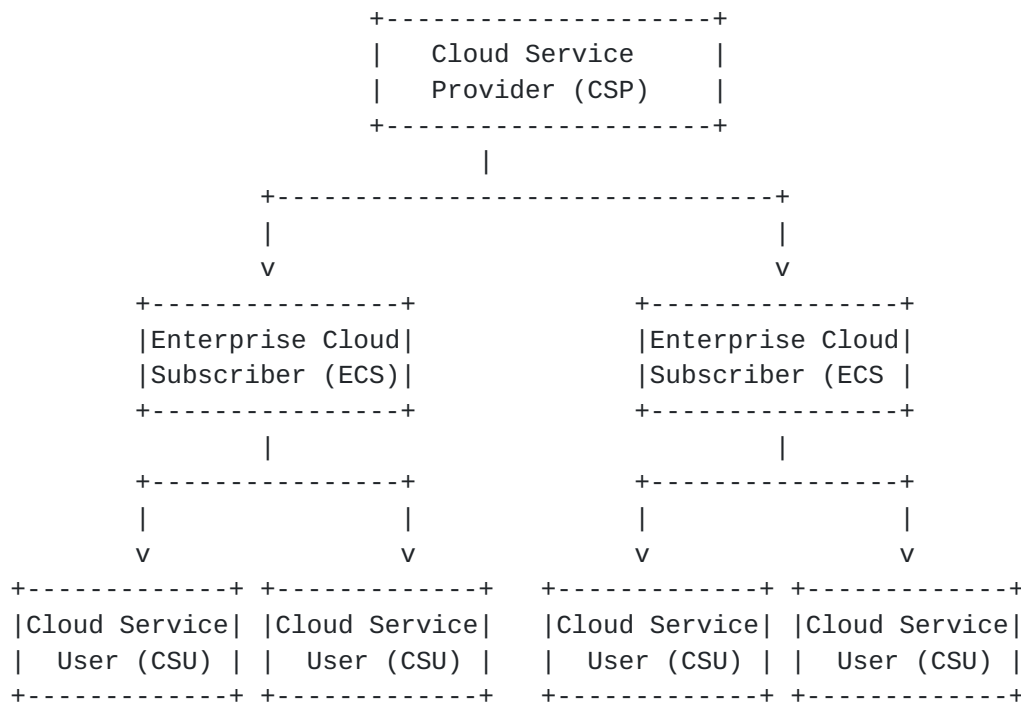
Figure 1: SCIM Actors
