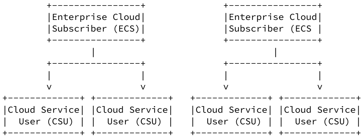
Figure 1: SCIM Actors
